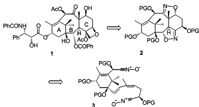
Scheme 1. Retrosynthetic analysis (PG = protecting group)
