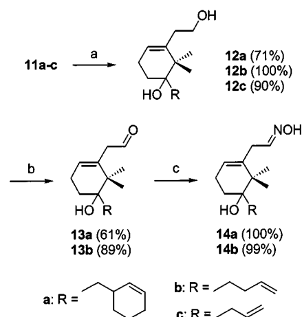
Scheme 4. Preparation of oximes 14a–b ; reagents and conditions: (a) \text{Bu}_4\text{NF} , THF, 0°C to room temp., 15 h; (b) \text{ClCO}_2 , DMSO, \text{CH}_2\text{Cl}_2 , -60°C, 15 min, then \text{Et}_3\text{N} , -60°C to room temp.; (c) \text{NH}_2\text{OH}/\text{HCl} , \text{Na}_2\text{CO}_3 , \text{CH}_2\text{Cl}_2/\text{H}_2\text{O} , 5 h, room temp.
