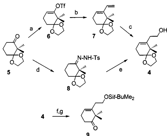
Scheme 3. Synthesis of ketone 9 ; reagents and conditions: (a) \text{KN}(\text{SiMe}_3)_2 , \text{PhNTf}_2 , THF, 0°C, 85%; (b) \text{Bu}_3\text{SnCH}=\text{CH}_2 , \text{Pd}(\text{PPh}_3)_4 cat., \text{LiCl} , THF, reflux, 95%; (c) 9-BBN, THF, reflux, then \text{H}_2\text{O}_2 , \text{NaOH} , THF/EtOH, 100%; (d) ref. [6] ; (e) t BuLi (4 equiv.), THF, -78 to 5°C, then ethylene oxide, THF, -78°C to room temp., 5 h, 67%; (f) \text{TsOH} , THF/ \text{H}_2\text{O} , reflux, 15 h, 99%; (g) t BuMe 2 SiCl, \text{Et}_3\text{N} , DMAP cat., \text{CH}_2\text{Cl}_2 , room temp., 1 h, 99%.
