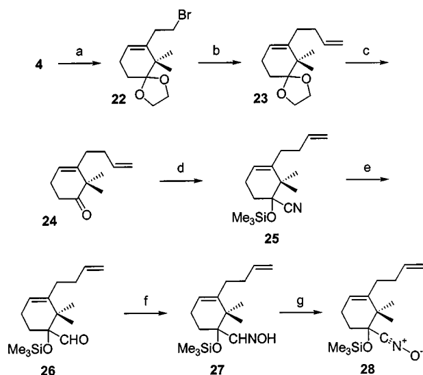
Scheme 8. Preparation of nitrile oxide 28 ; reagents and conditions: (a) \text{CBr}_4 , \text{PPh}_3 , \text{CH}_2\text{Cl}_2 , room temp., 100%; (b) vinylMgBr, CuI, THF, 0^\circ\text{C} to room temp., 95%; (c) TsOH, THF, \text{H}_2\text{O} , 100%; (d) \text{Me}_3\text{SiCN} , \text{ZnI}_2 , \text{CH}_2\text{Cl}_2 , 0^\circ\text{C} to room temp., 85%; (e) DIBAL-H, \text{Et}_2\text{O} , 0^\circ\text{C} , 70%; (f) \text{NH}_2\text{OH}\cdot\text{HCl} , pyridine/ \text{EtOH} , 100%; (g) \text{NaOCl} , \text{H}_2\text{O}/\text{CH}_2\text{Cl}_2 , 95%
