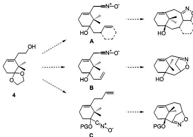
Scheme 2. Strategies for the formation of the ring B of taxanes by intramolecular nitrile oxide cycloaddition (PG = protecting group)
