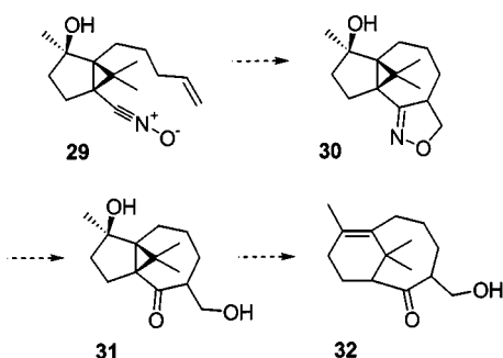
Scheme 9. Modification of the strategy planned
