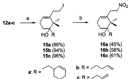
Scheme 5. Preparation of nitro compounds 16a–c ; reagents and conditions: (a) \text{PPh}_3 , imidazole, \text{I}_2 , \text{Et}_2\text{O}/\text{CH}_3\text{CN} , 0^\circ\text{C} to room temp., 4 h; (b) \text{NaNO}_2 , DMF, room temp.
