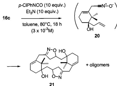
Scheme 7. Cycloaddition from nitro compound 16c
