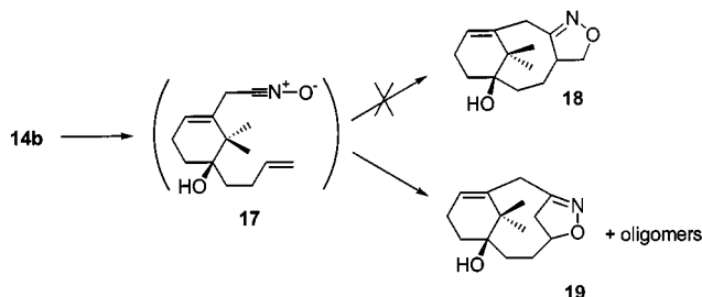
Scheme 6. Cycloaddition from oxime 14b
